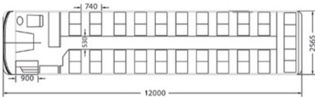
Suggested Seating Layout, Dimensions in mm
